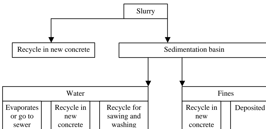
Figure 3.10 Treatments for slurry. Illustration taken from fib (2003b). 29
