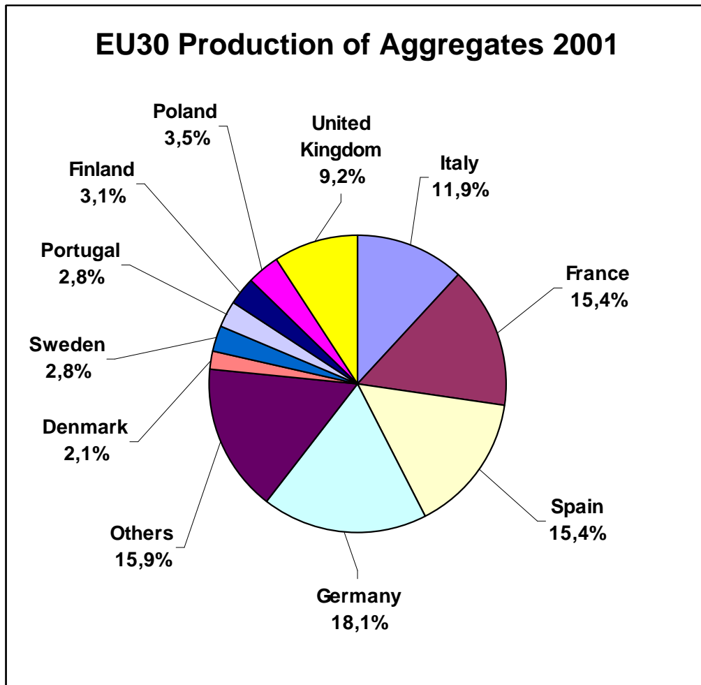
Figure 2.3 Production of Aggregates (2001) – Percentage Distribution. (Source: the European Mineral Statistics 1997–2001 6 ).
