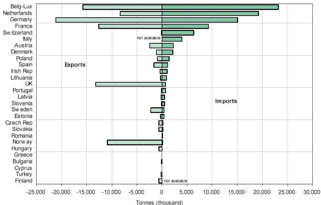
Figure 2.4 Aggregates trade in 2001. (Source: the European Mineral Statistics 1997–2001 6 ).
